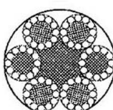
6x12+7FC
