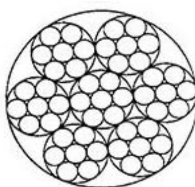
6x7+IWS
