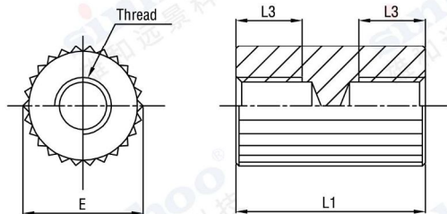
RSDD Round Female to Female standoffs
