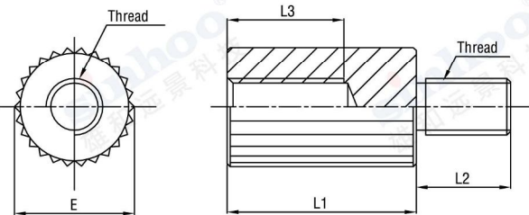
RSD Round Male-Female Standoffs
