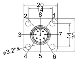
8pin
