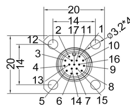
17pin
