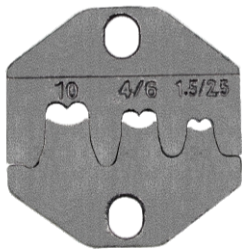
Mold A
