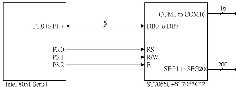
8-bit interface
