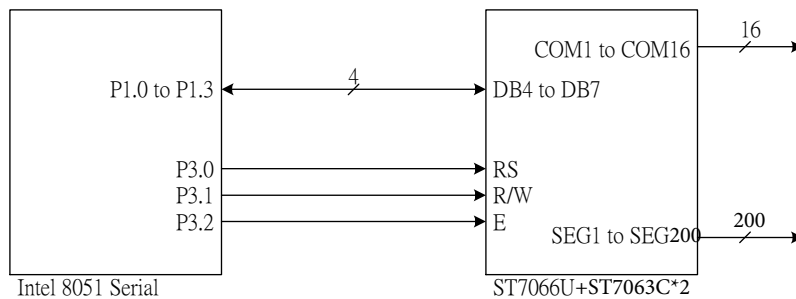
4-bit interface
